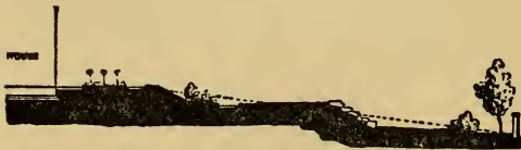
Fig. 33.—Terracing — sectional view
